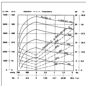
MEC6500M
