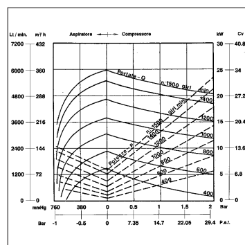
MEC5000P-D-H
