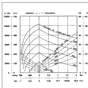
WPT600 P-D-H
