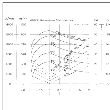
KTS960 P-D-H
