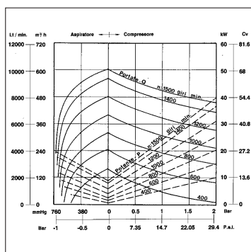
WPT480 P-D-H
