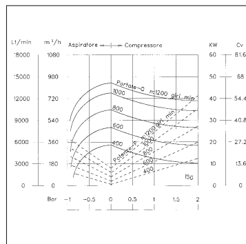
KTS840 P-D-H
