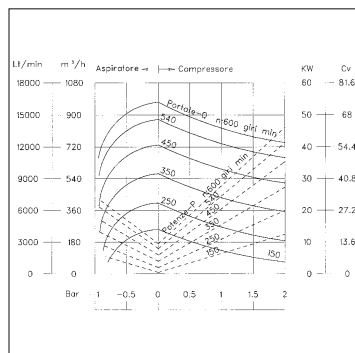
KTS960 P-D-H
