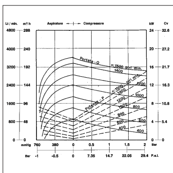
MEC3000P-D-H
