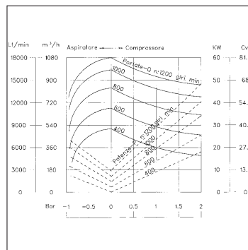
KTS1080 P-D-H
