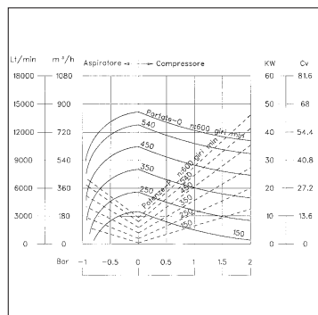
KTS840 P-D-H
