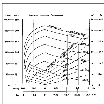
MEC4000P-D-H
