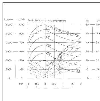
KTS1080 P-D-H
