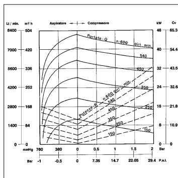
MEC8000M
